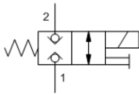
M-Control, C-Poppet
