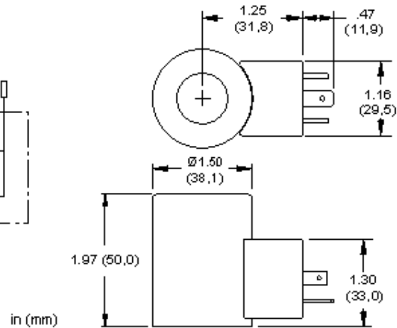
DC COIL
