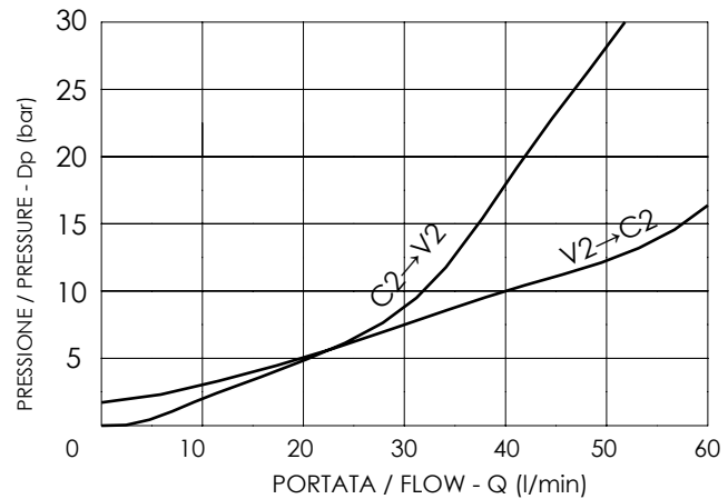
CURVE CARATTERISTICHE / PERFORMANCE CURVES
