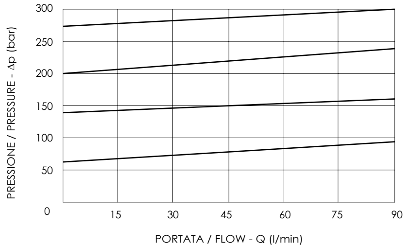
CURVE CARATTERISTICHE / PERFORMANCE CURVES
