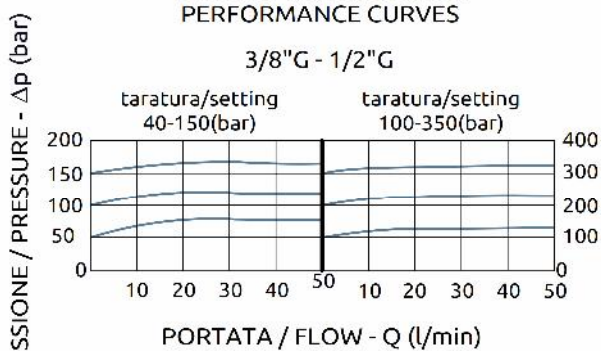
CURVE CARATTERISTICHE PERFORMANCE CURVES
