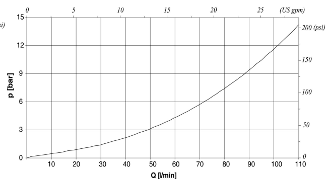
Typical Pressure drop vs. Flow characteristic P \rightarrow U
