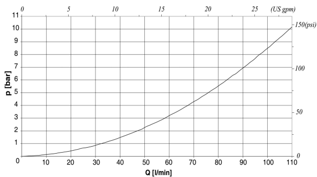
Typical Pressure drop vs. Flow characteristic P \rightarrow T
